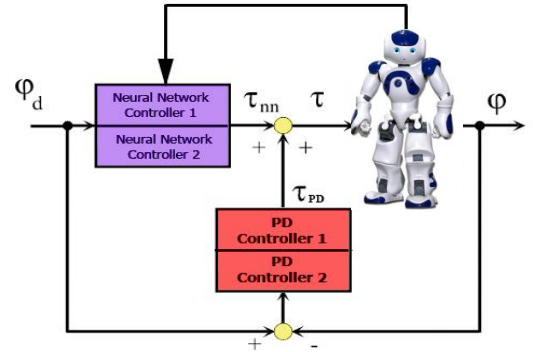
Fig.6. Proposed neural control system for walking robot.
