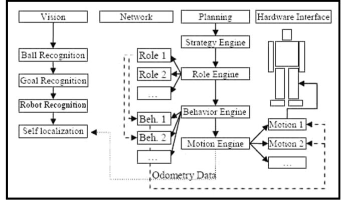
Fig. 4. Structure of the control software
