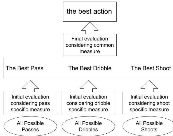
Fig. 3. Two phase decision making mechanism
