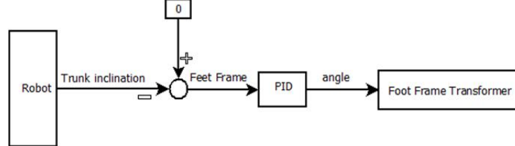
Fig. 3: Active Balance controller
