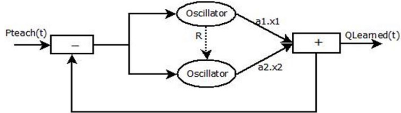
Fig 6. Schematic view of network of adaptive Hopf oscillators as a programable CPGs network, where P_{teach}(t) is the genrated trajectory by Fourier Series
