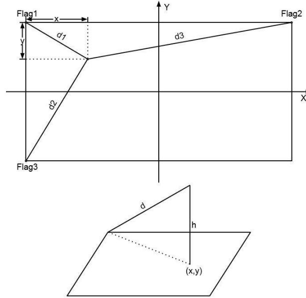
Fig.2. Self-Location and Calculating the Height
