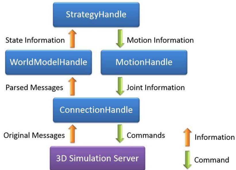
Fig.1. HfutEngine3D main running flow in about one cycle
