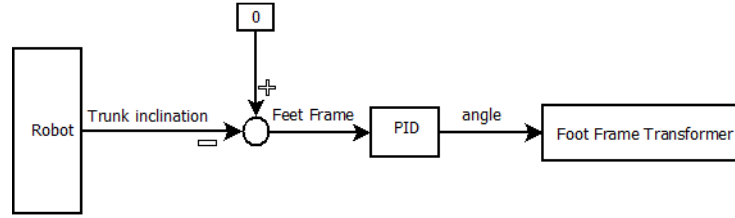
Fig. 3: Active Balance controller
