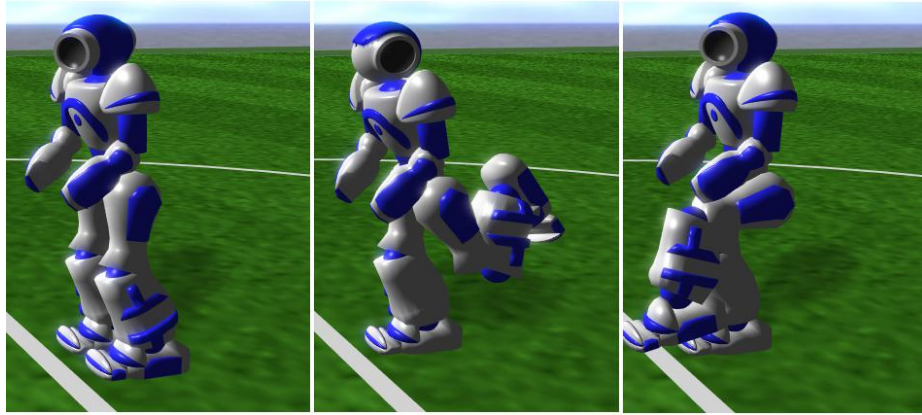
Fig. 1. kick skill
