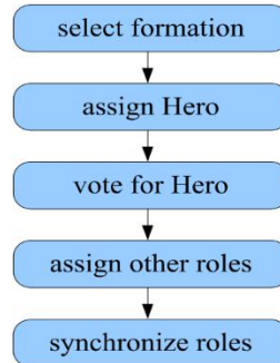
Fig. 4. Flow chart of assigning roles
