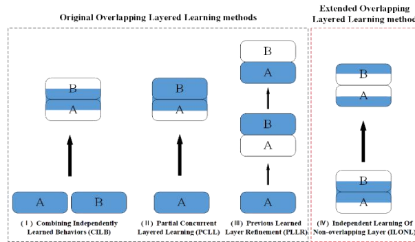
Fig. 2. Independent Learning Of Non-overlapping Layer
