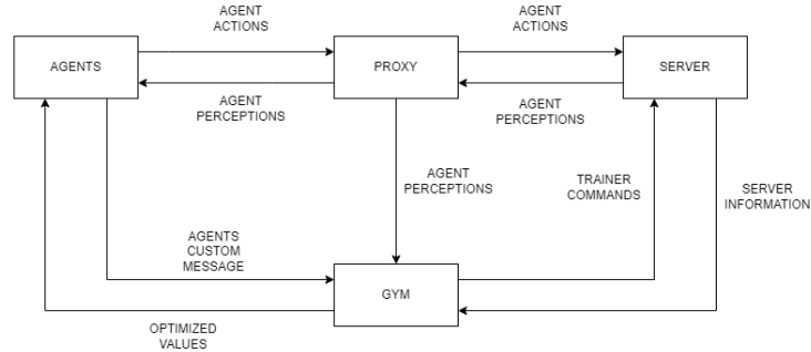
Fig. 1. BahiaRT Gym Process Architecture
