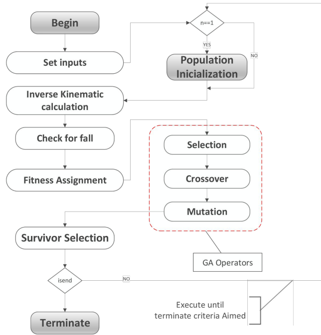
Fig. 3. Walking algorithm based on inverse kinematics with optimization by genetic algorithm [1]
