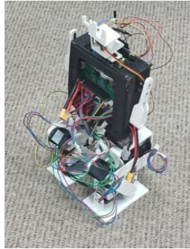
Fig. 2. HRPIME-23: Humanoid Robotic Platform
